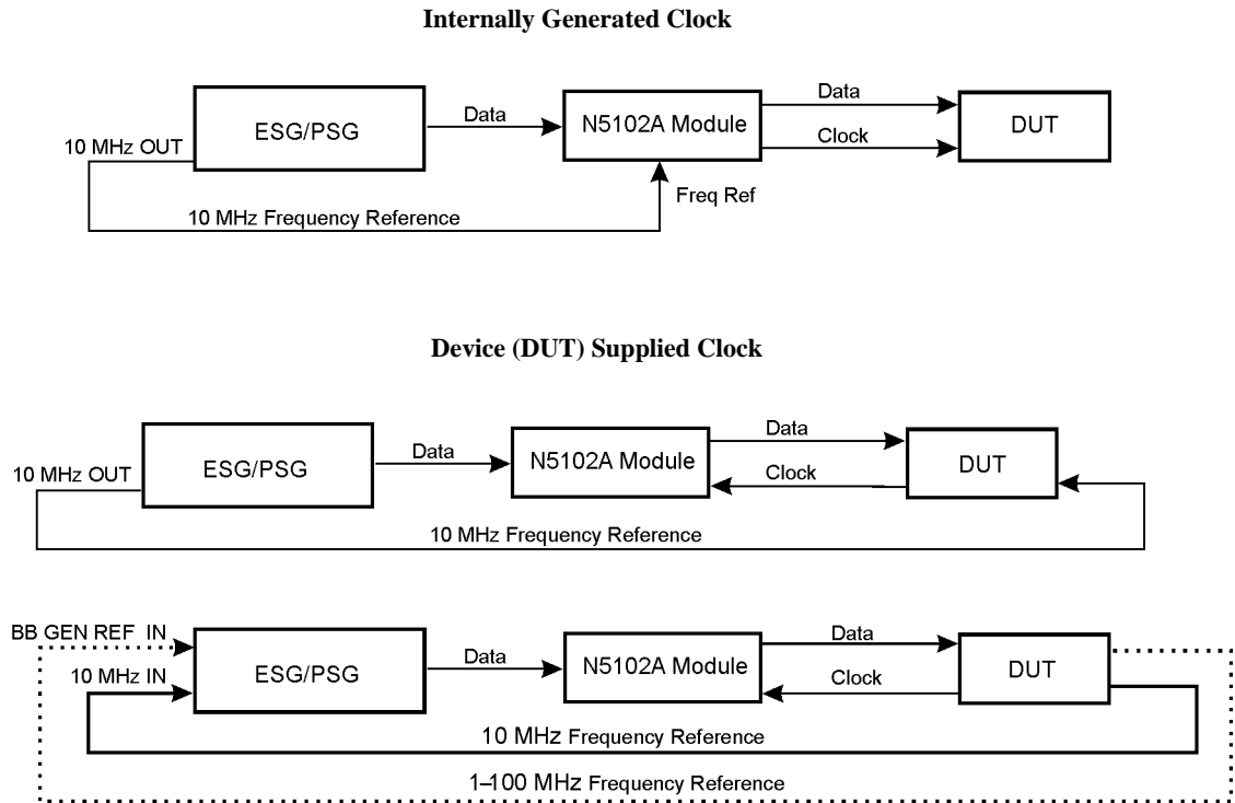
Figure 12-3 Frequency Reference Setup Diagrams for the N5102A Module Clock Signal
