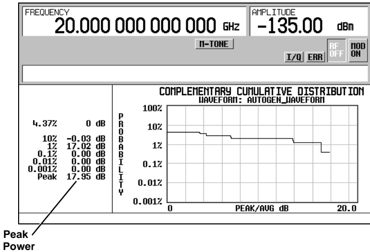
Figure 9-7 CCDF Plot with Fixed Phase Set
