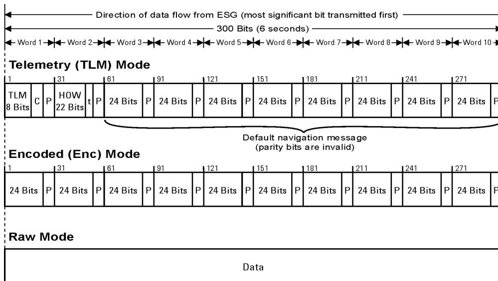
Figure 8-4 Subframe Structures
